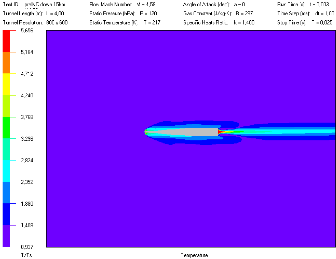
Altitude 15 km, M4.58, surface temperature is about 550 deg on the cone.
