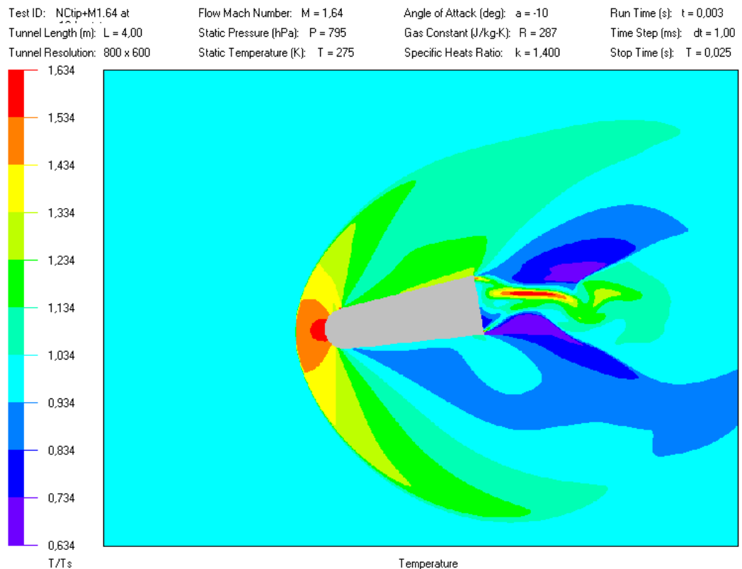
The NC tip at M1.64, attack angle -10\text{deg} . Temperature displacement in case of wobbling of 20\text{deg} total amplitude.
