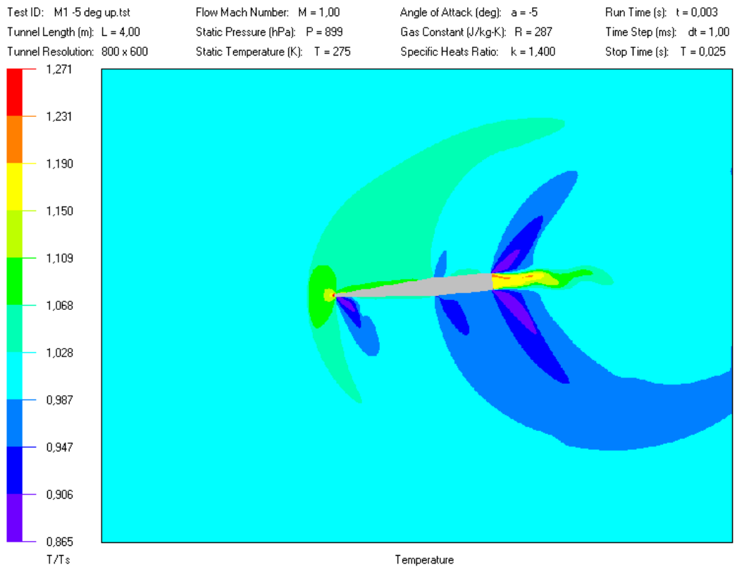
M1 at -5 deg. During possible wobbling, the temperature profile is changing. I am not expecting any wobbling at supersonic velocities; if there would be any, the aerodynamic loads would destroy the vehicle immediately.
