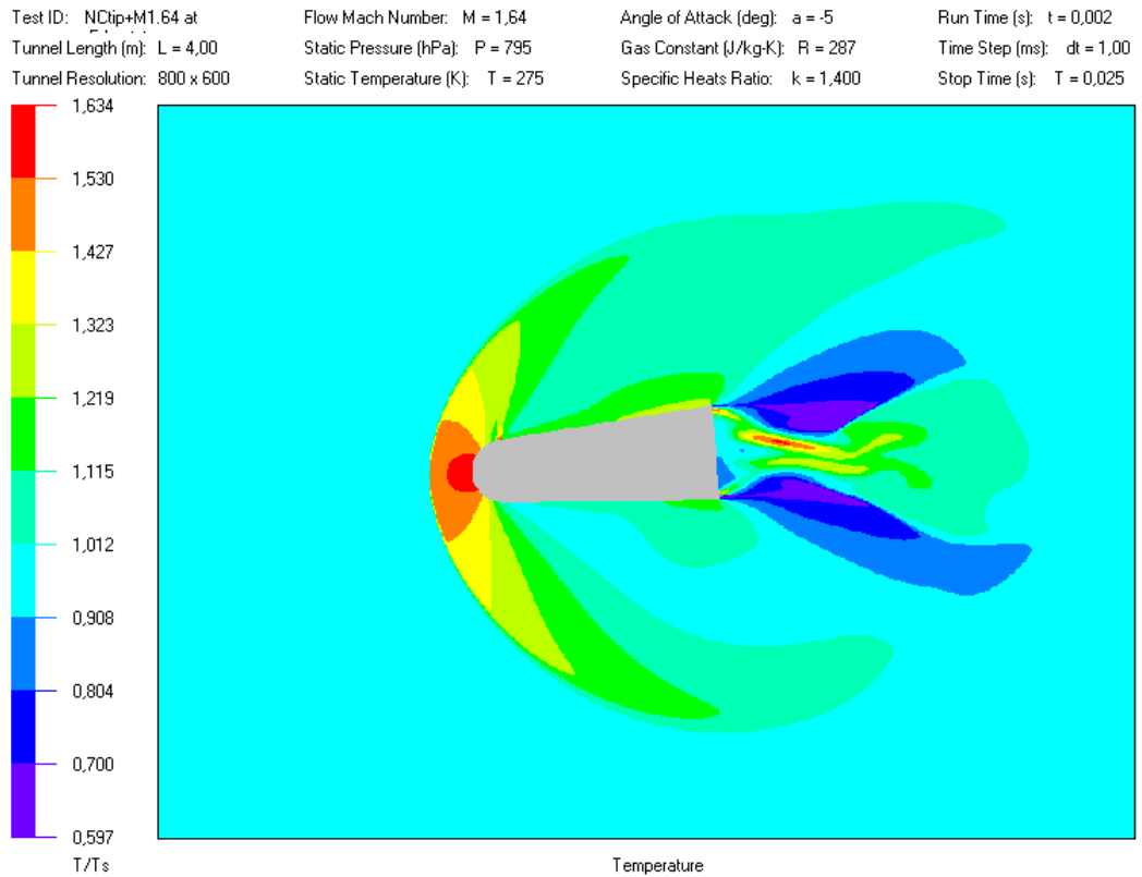
The NC tip at M1.64, attack angle -5\text{deg} . Temperature displacement in case of wobbling about 10\text{deg} of total amplitude.
