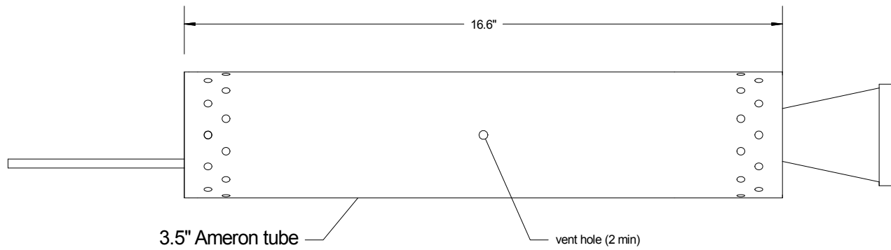
Proposed test setup for assessing propellant structure behaviour under pressure loading
